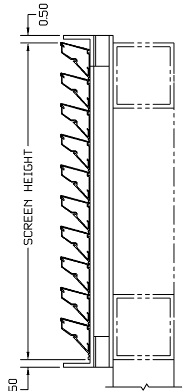
VERTICAL SECTION
