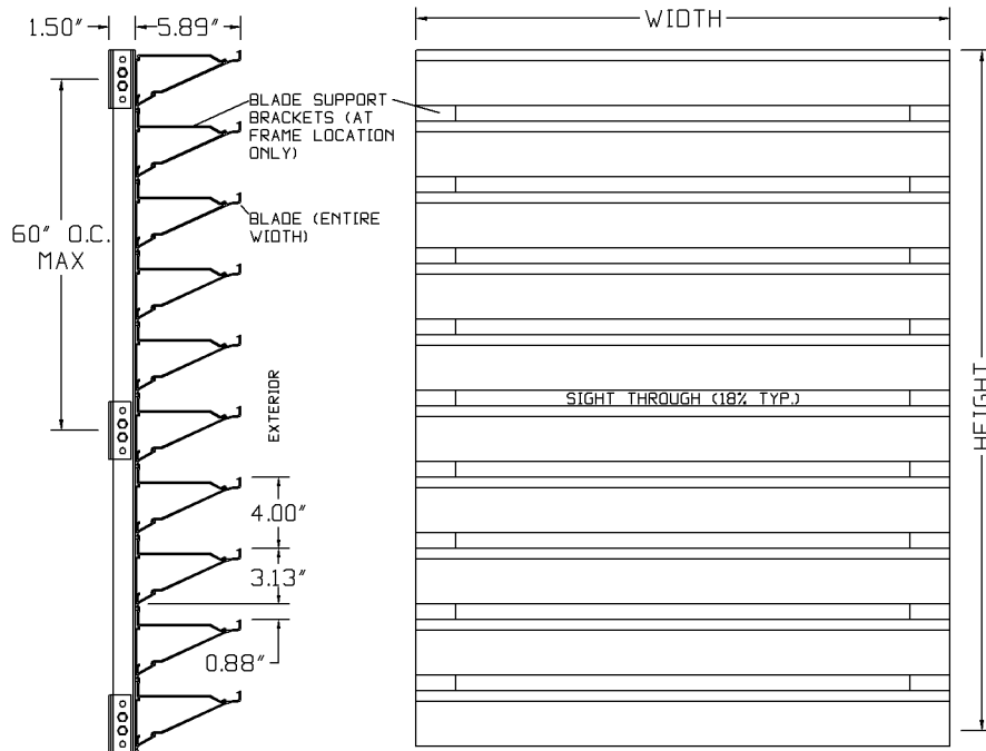
SECTION VIEW
