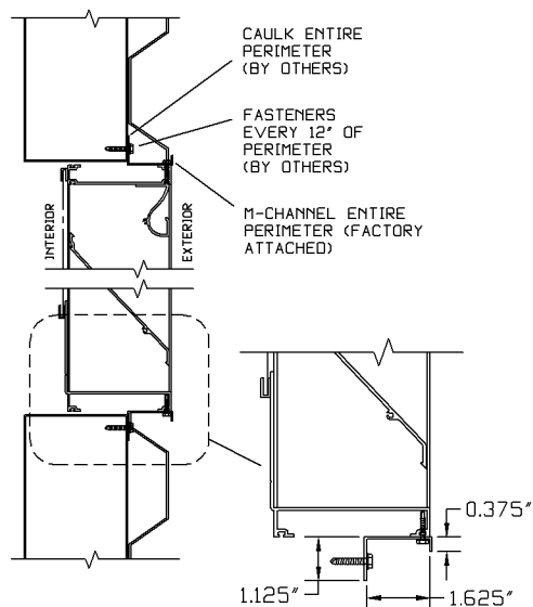
"M" CHANNEL FRAME (NOT AVAILABLE FOR RADIUS OR ROUNDS)
