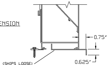
CHANNEL "C" FRAME (OPTIONS)
