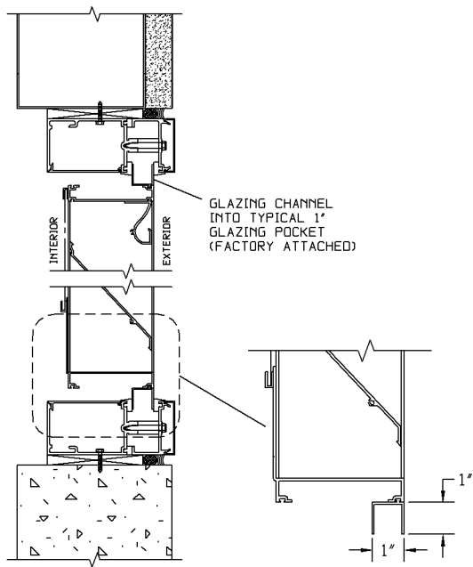
"J" CHANNEL FRAME
