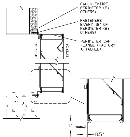
CAP "Z" FRAME
