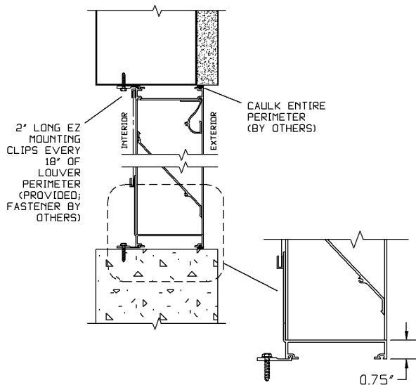
CHANNEL "C" FRAME (STANDARD)
