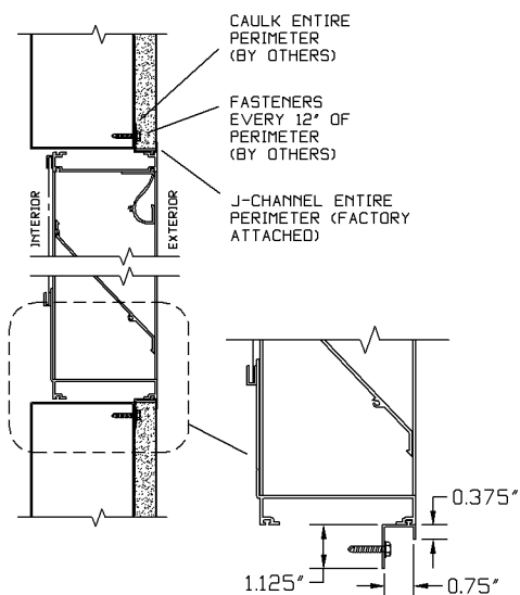
"J" CHANNEL FRAME
