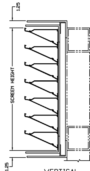
VERTICAL SECTION
