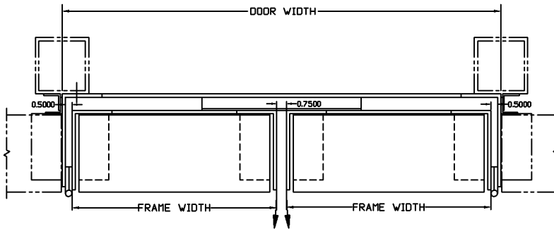
HORIZONTAL SECTION
