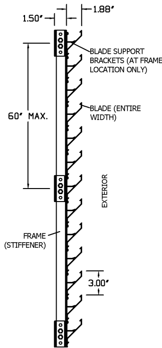
SECTION VIEW
