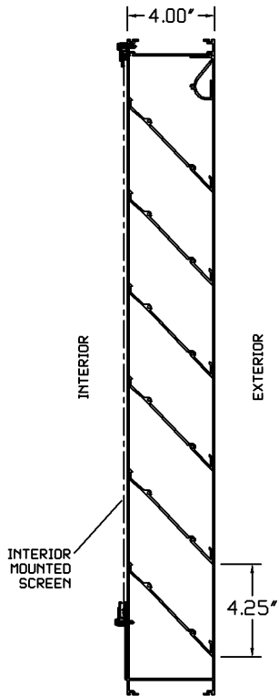
SECTION VIEW
