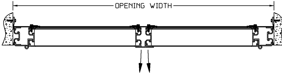
HORIZONTAL SECTION
