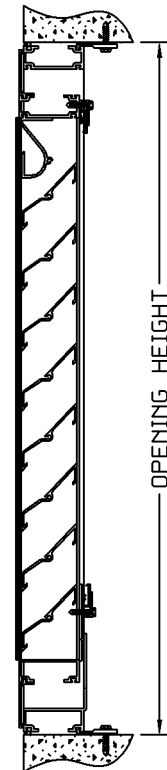
VERTICAL SECTION
