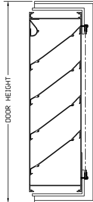
VERTICAL SECTION
